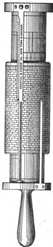
FIG. 13.—C. FULLER'S SLIDE RULE.
