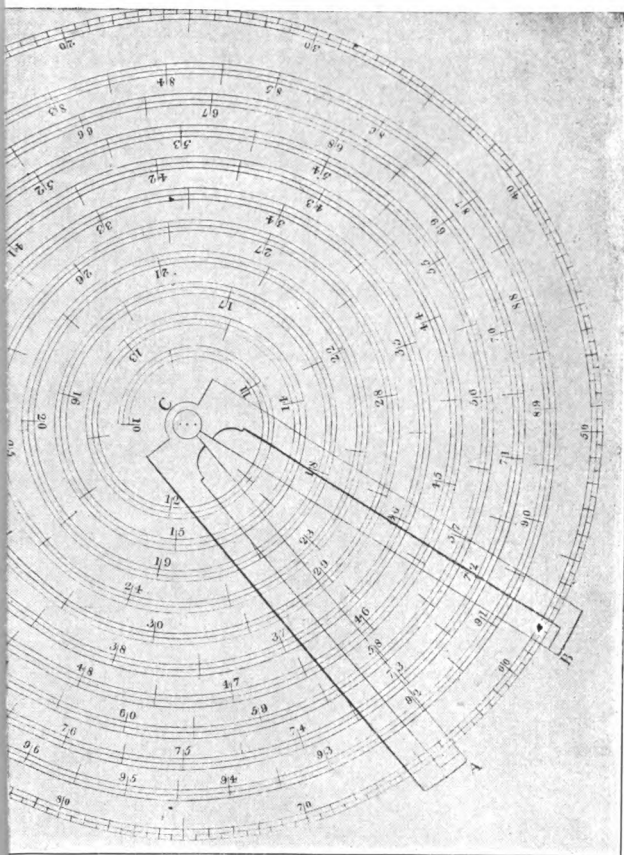
NICHOLSON'S SPIRAL SLIDE RULE OF 1797.
