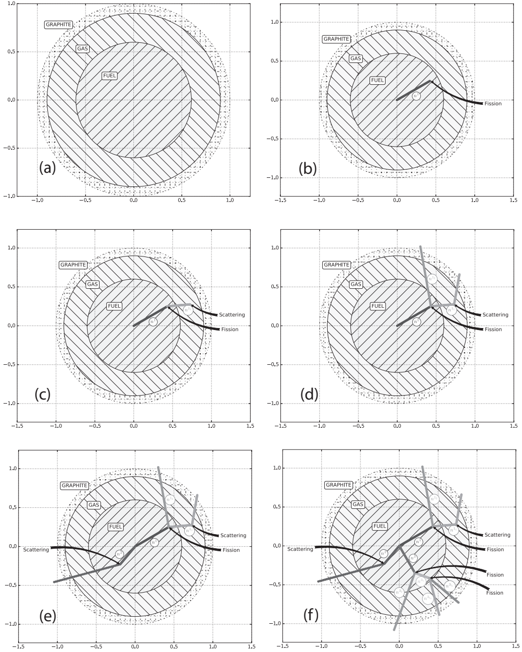
Fig. 6. – An example of the Fermi wheel used to follow the fate of the genealogy of source neutrons n^1 , n^2 , n^3 in a cell of a nuclear reactor.
